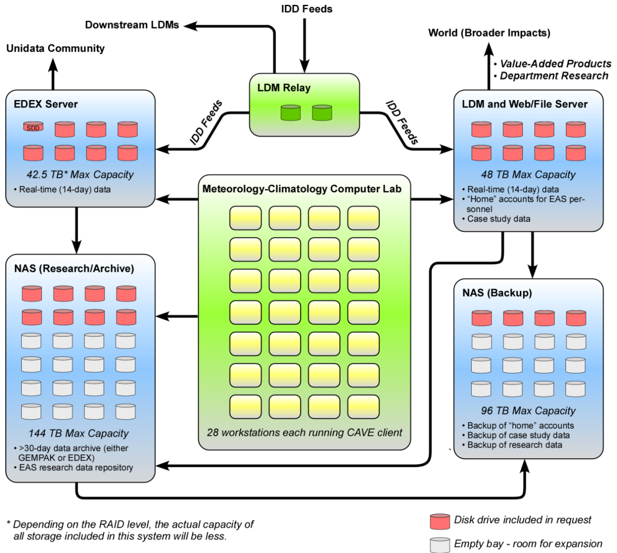
Figure 3. Schematic of the proposed system. Blue boxes indicate components included in this request while green boxes represent existing infrastructure. Cylinders denote disk bays; pink disk bays are included in this request.
